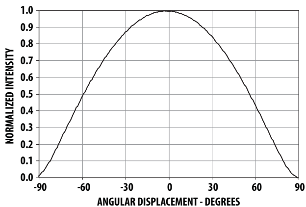
Figure 10. Radiation Pattern
