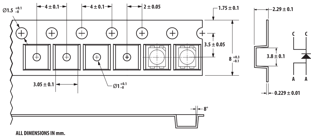
Figure 15. Tape Dimensions
